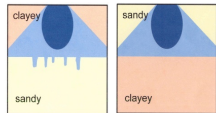
Figure 8. (left) With clayey soil over sandy soil, water is slow to leave to leave the small pore space of the clay. (right) With Sandy over clayey soil, water is slow to move into the small pore space of the clay.
