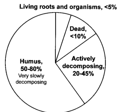
Make-up of soil organic matter
