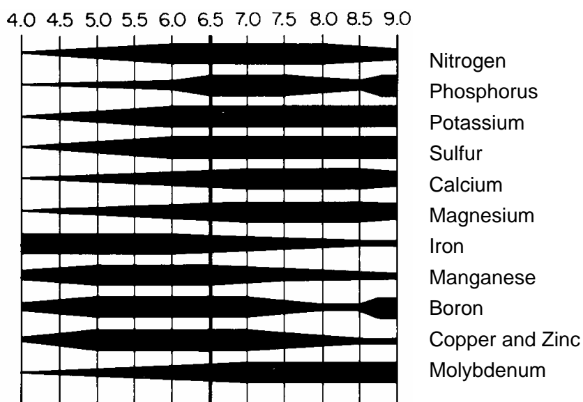
Figure 1. Availability of nutrients based on soil pH
